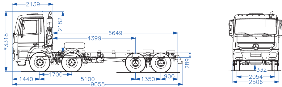
Measurements for vehicle in unladen condition
