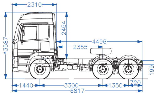
Sleeper Cab
